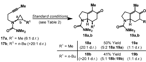
Scheme 3. Substitution of the Aminocyclopropane
